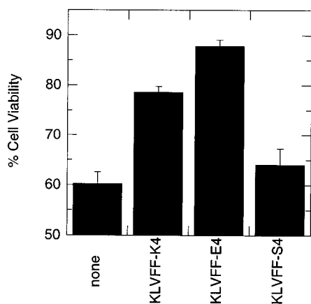
FIGURE 5: Effect of hybrid peptides with variable-charged disrupting domains on cellular toxicity of A\beta solutions. A\beta alone or with the indicated peptide was incubated for 2 days at 37 °C, and then added to plated PC-12 cells for 1 day. The A\beta concentration in wells was 25 \mu M, and the A\beta :hybrid molar ratio was 1:1. Cellular viability was assessed with the MTT assay. Each bar represents the mean \pm standard deviation of results from two to five separate runs, with seven replicates per run.
